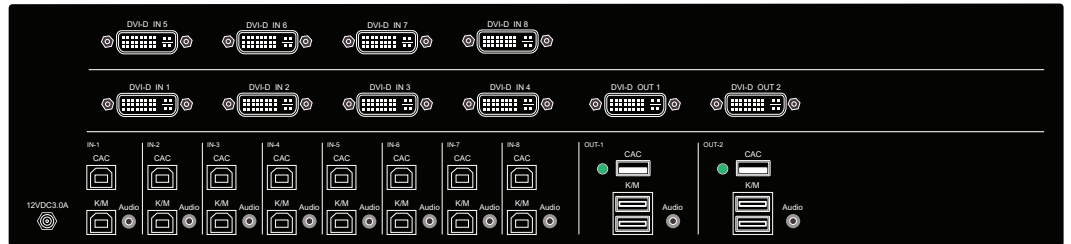
Figure 5-2: SS8P-DVI-8X2-UCAC Rear panel
