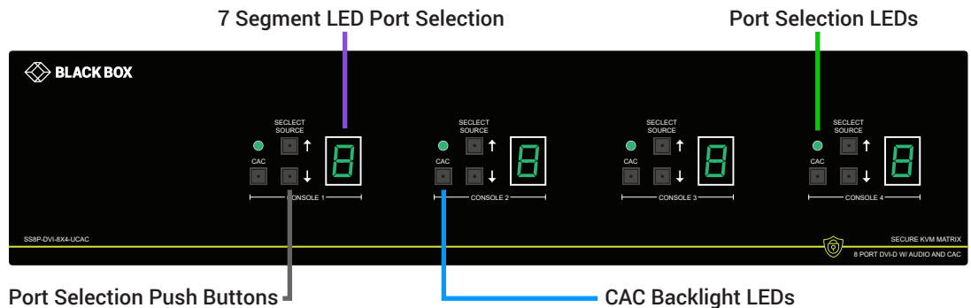
Figure 4-1: SS8P-DVI-8X4-UCAC Front panel
