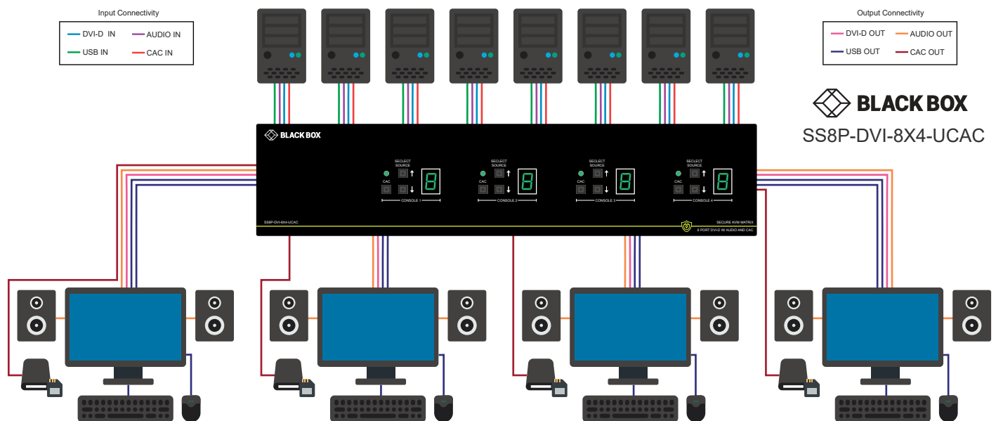
Figure 7-1: SS8P-DVI-8X4-UCAC
