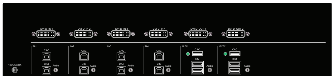
Figure 5-6: SS8P-DVI-4X2-UCAC Rear panel
