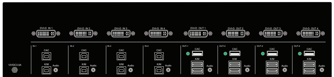
Figure 5-4: SS8P-DVI-4X4-UCAC Rear panel
