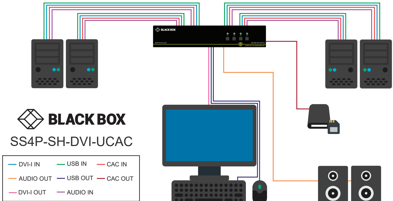
Figure 6-1: SS4P-SH-DVI-UCAC
