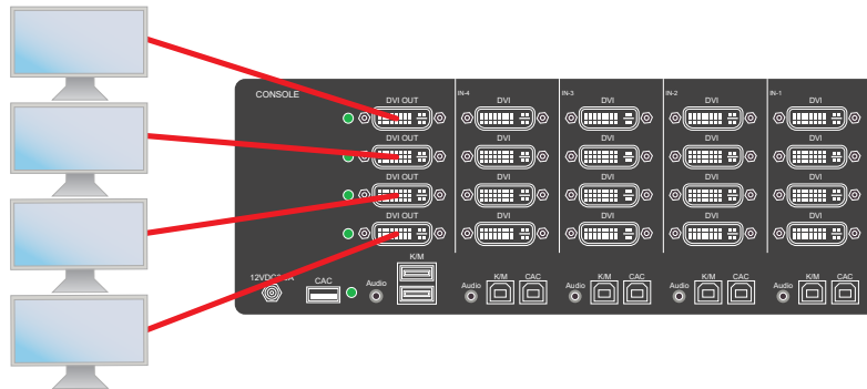
Figure 7-2: SS4P-QH-DVI-UCAC
