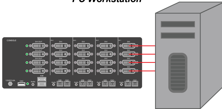
Figure 7-1: SS4P-QH-DVI-UCAC
