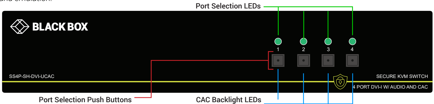
Figure 4-1: SS4P-SH-DVI-UCAC Front panel
