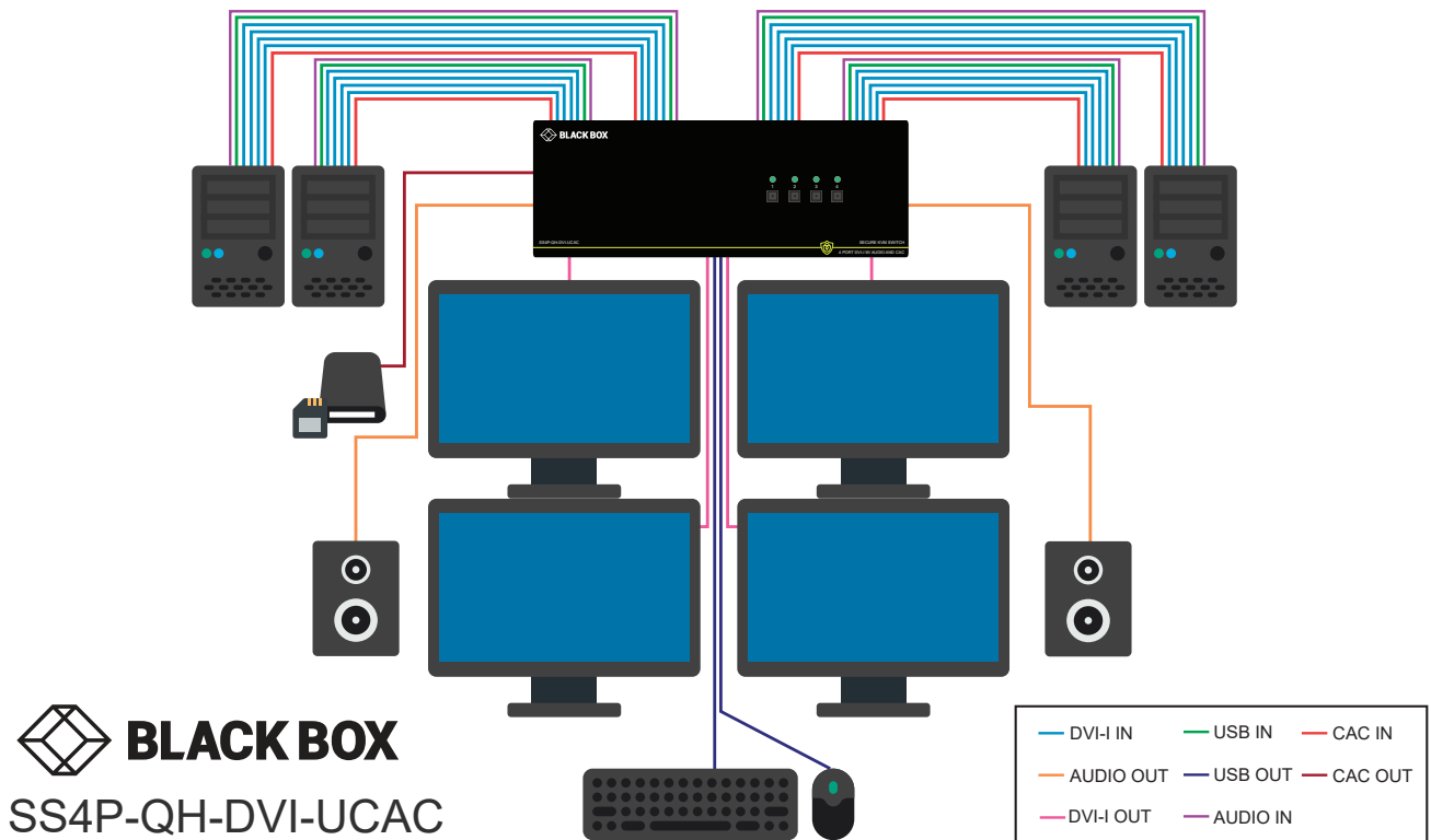
Figure 8-1: SS4P-QH-DVI-UCAC
