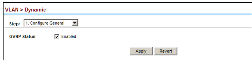
Figure 86: Configuring Global Status of GVRP
