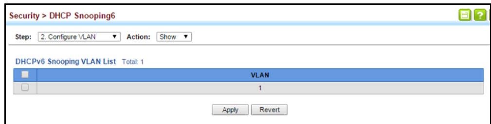
Figure 231: Showing VLANs Enabled for DHCPv6 Snooping
