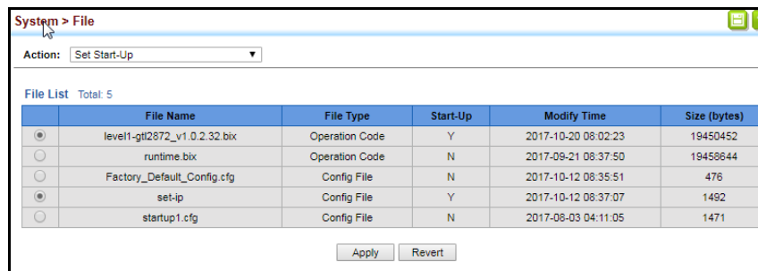
Figure 10: Setting Start-Up Files
