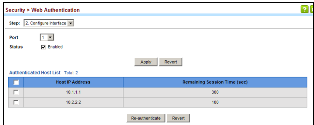
Figure 192: Configuring Interface Settings for Web Authentication
