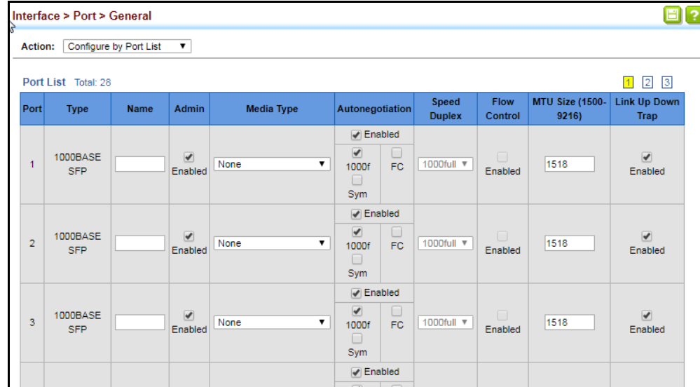
Figure 32: Configuring Connections by Port List
