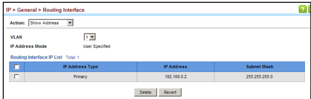
Figure 433: Showing the Configured IPv4 Address for an Interface
