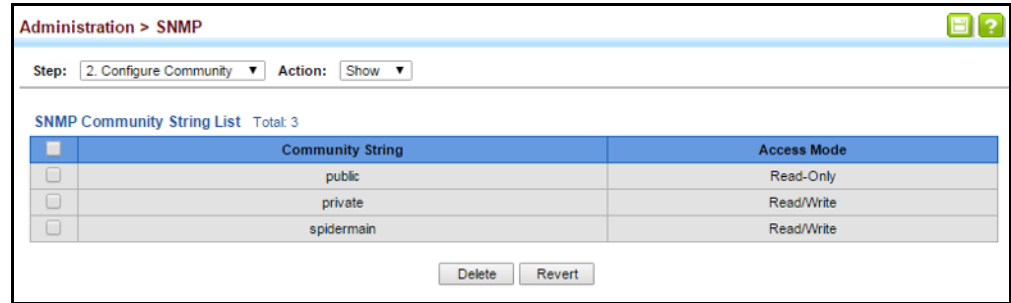
Figure 266: Showing Community Access Strings
