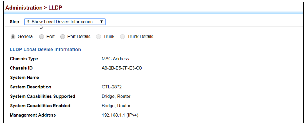
Figure 258: Displaying Local Device Information for LLDP (Port)
