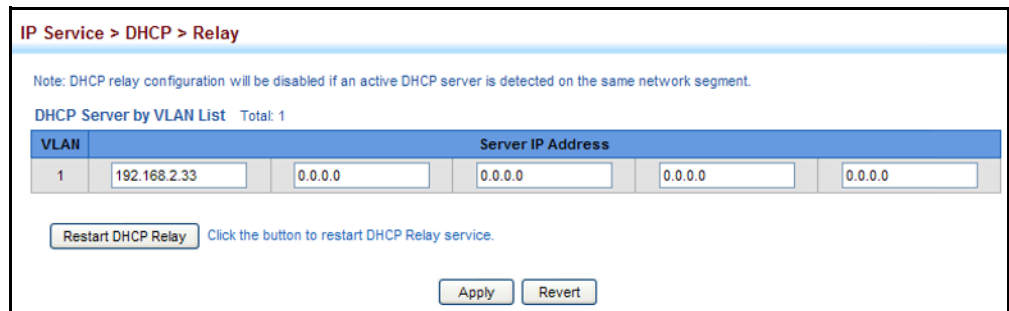
Figure 458: Configuring DHCP Relay Service
