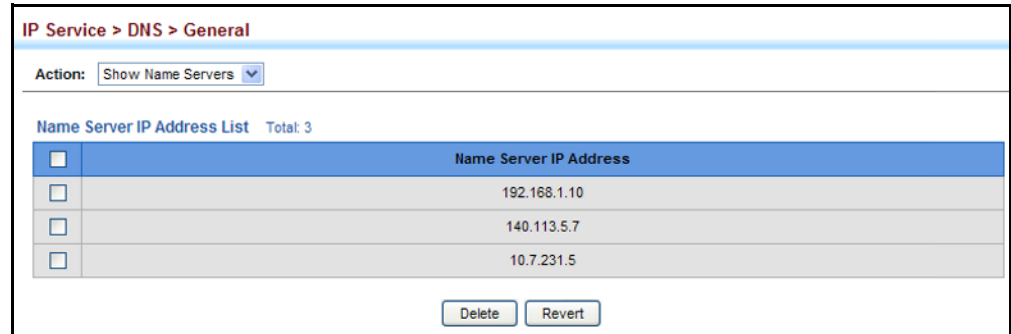
Figure 452: Showing the List of Name Servers for DNS
