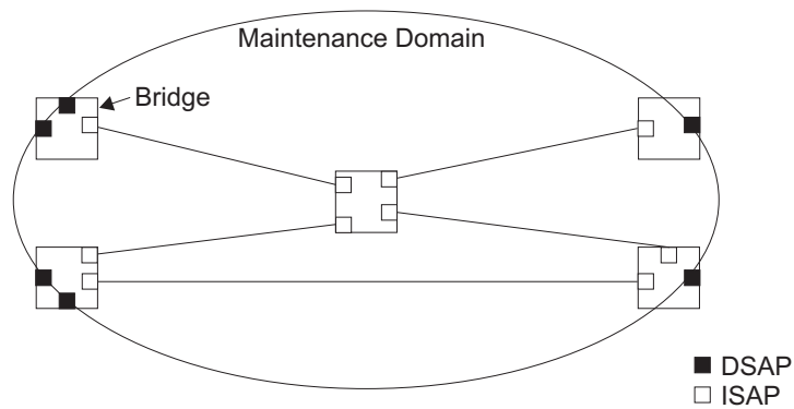
Figure 325: Single CFM Maintenance Domain
