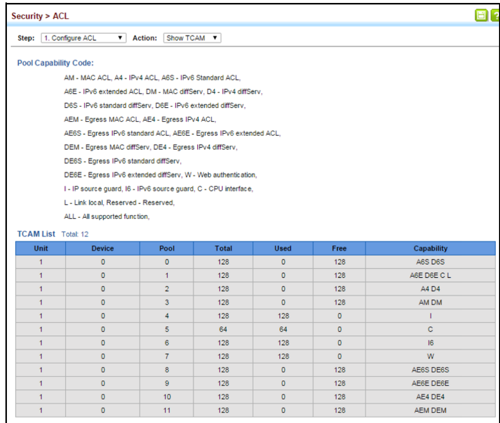
Figure 206: Showing TCAM Utilization
