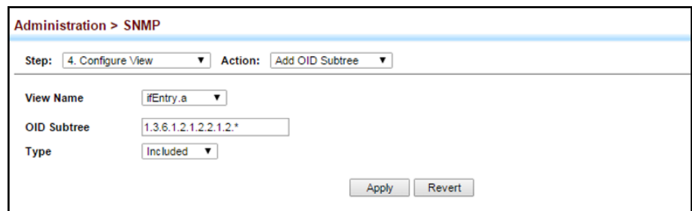
Figure 272: Adding an OID Subtree to an SNMP View
