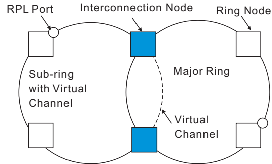
Figure 312: Sub-ring with Virtual Channel
