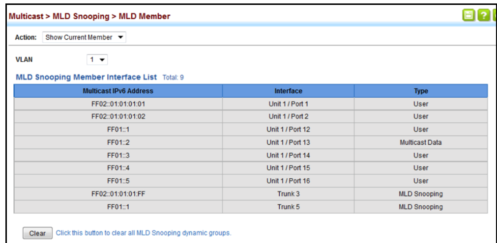
Figure 388: Showing Current Interfaces Assigned to an IPv6 Multicast Service
