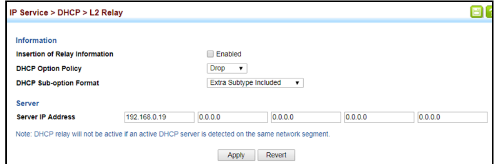
Figure 460: Configuring DHCP Relay Information Option 82 Service
