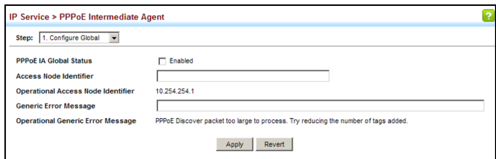
Figure 462: Configuring Global Settings for PPPoE Intermediate Agent
