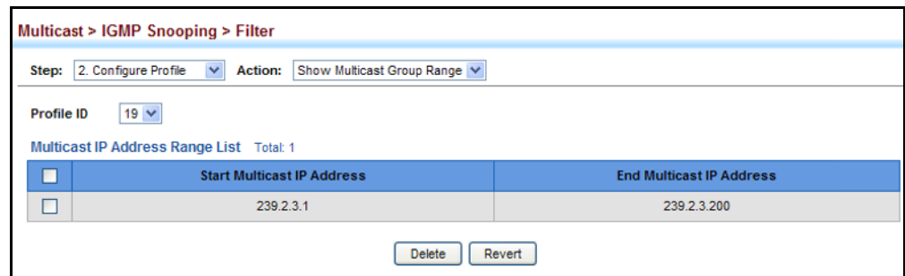
Figure 379: Showing the Groups Assigned to an IGMP Filtering Profile
