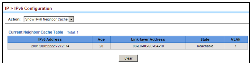
Figure 439: Showing IPv6 Neighbors
