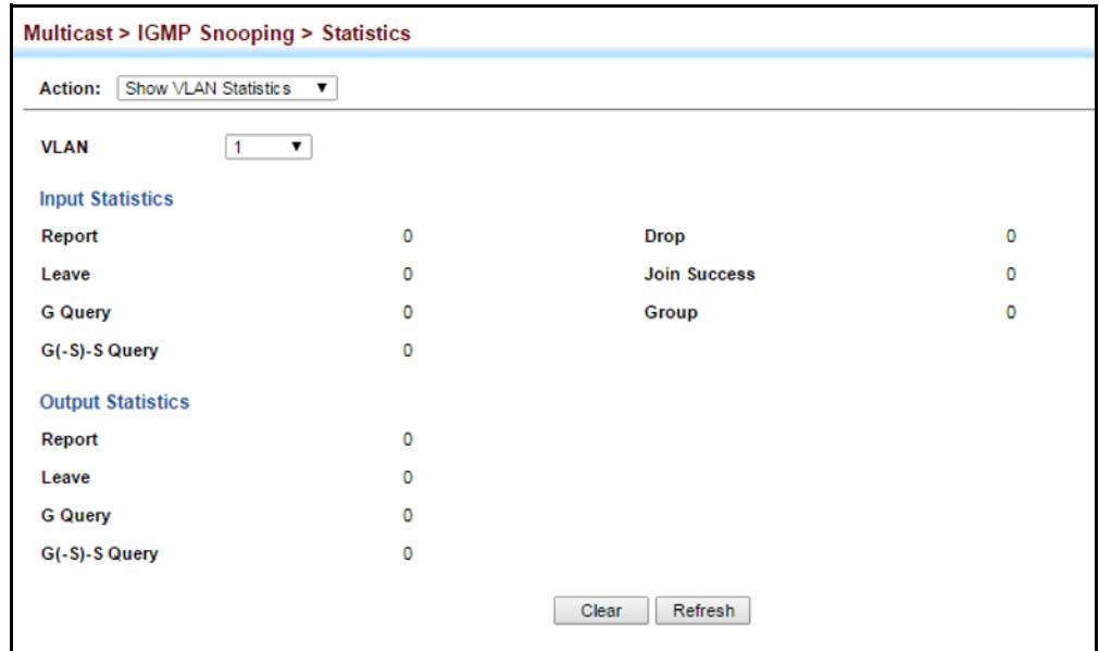
Figure 373: Displaying IGMP Snooping Statistics – VLAN
