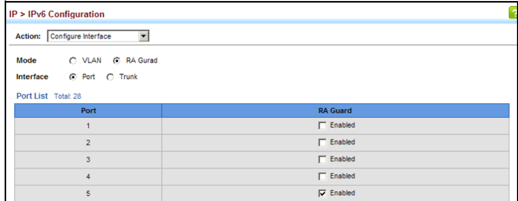
Figure 436: Configuring RA Guard for an IPv6 Interface
