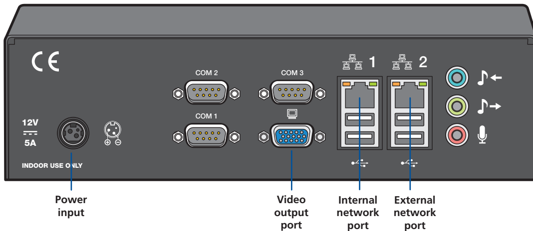
Figure 2-5. ServSwitch iPATH unit - rear panel. During normal use, only the network and power connections are used.
