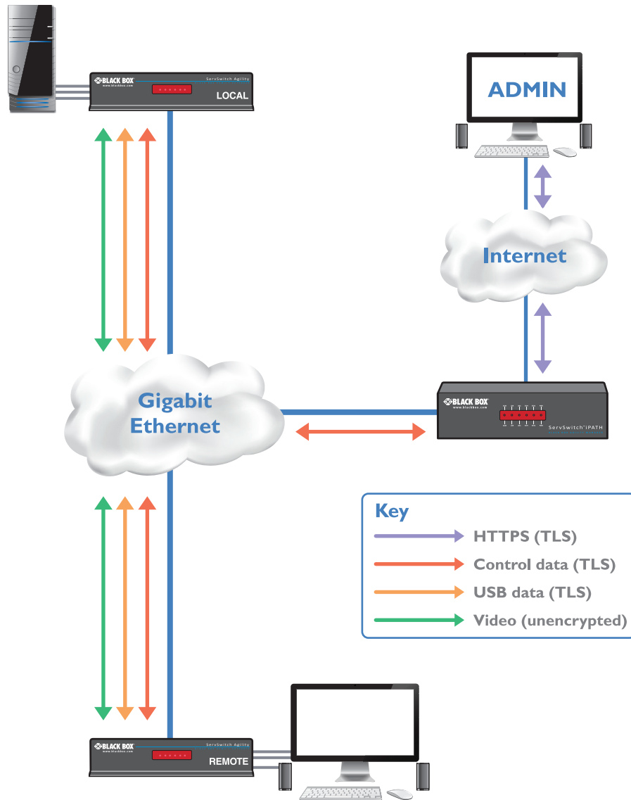
Figure 2-2. Transport Layer Security data diagram
