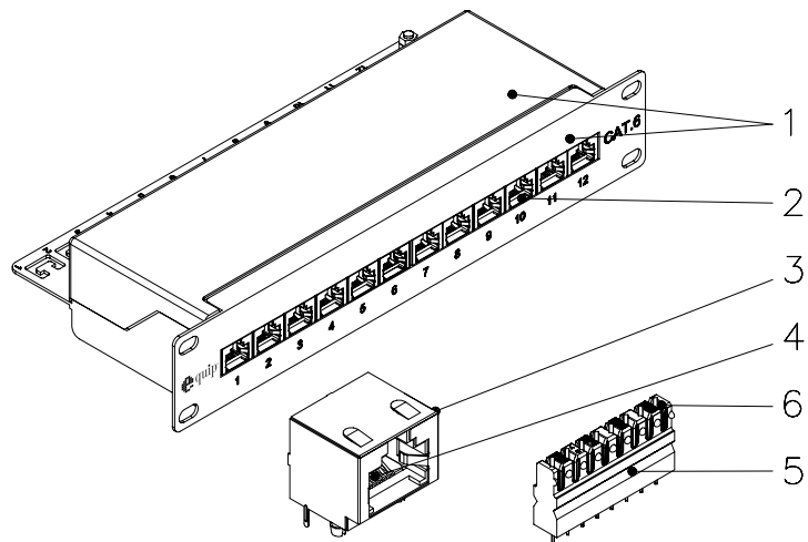
RJ45 RIGHT ANGLE JACK IDC (KDA) Krone 45°-110 Dual SCALE 1/4
